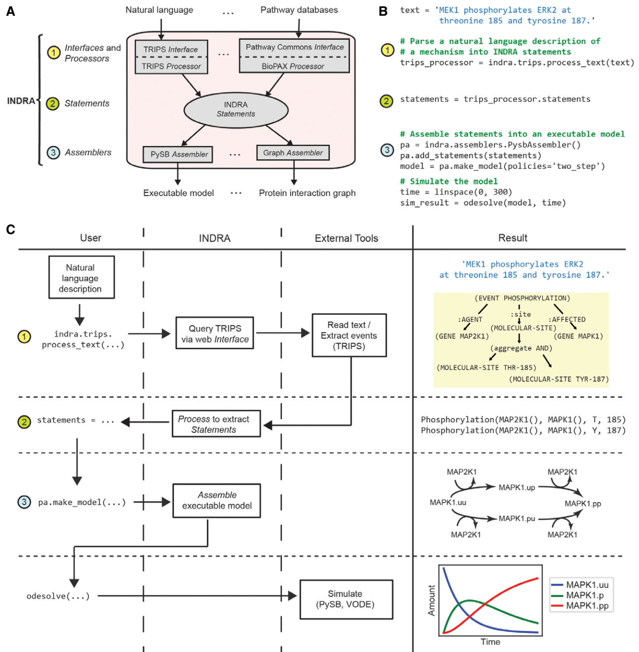
Figure 1. Building a model from natural language with INDRA.
