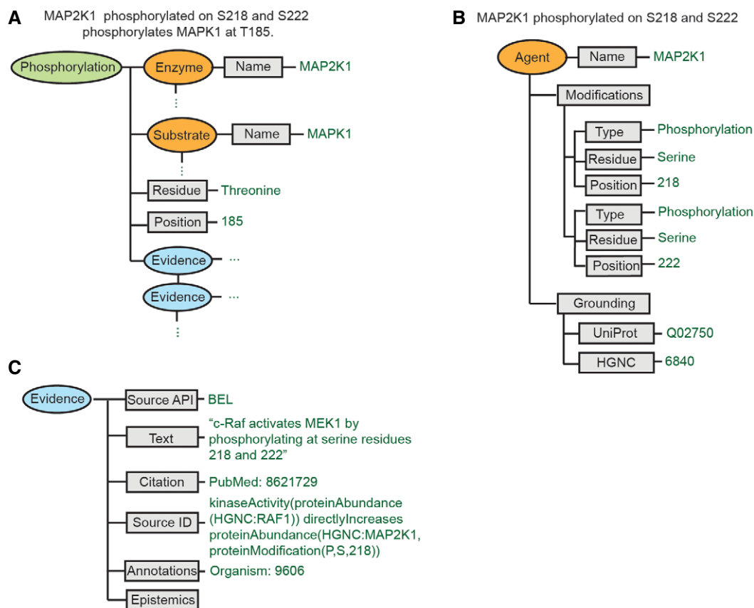
Figure 2. INDRA Statements represent molecular agents and biochemical mechanisms.
