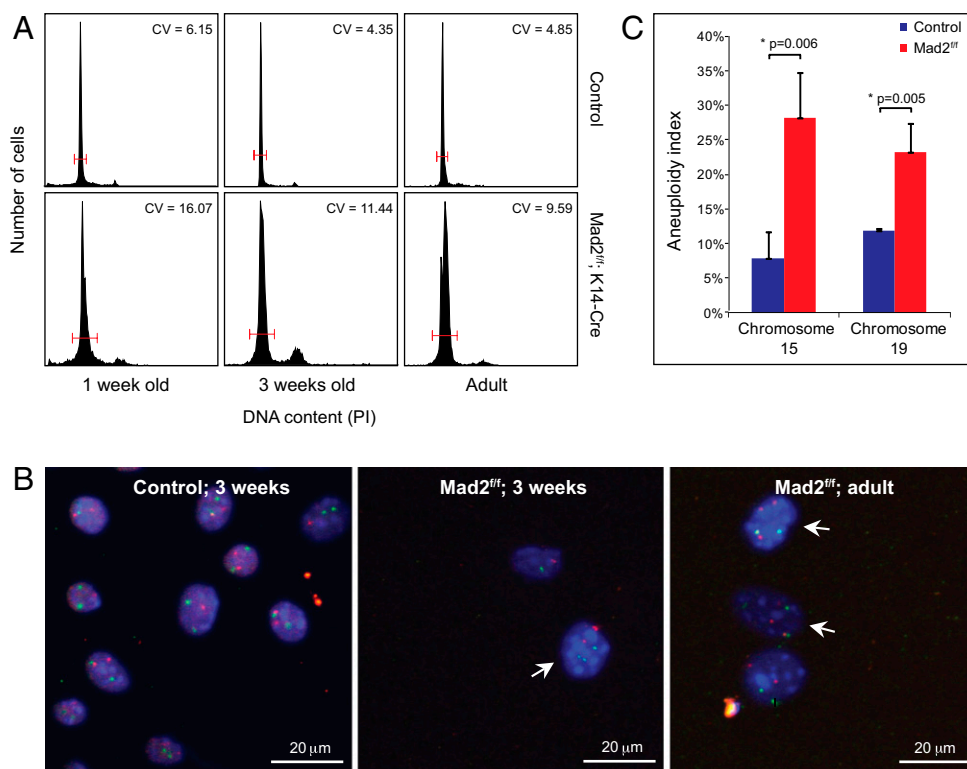
Fig. 2. Krt14-Cre ; Mad2 conditional mice display dramatic aneuploidy in the epidermis. (A) DNA content distribution in control and Mad2 -deficient epidermal cells in neonates and adults. The CV is used as a measure of the variance of DNA content within the G1 peak. (B) Interphase FISH for chromosomes 15 (red) and 19 (green) on freshly isolated control and Mad2 -deficient keratinocytes. (C) Percentage of cells showing more than two copies of chromosome 15 or 19 assessed by interphase FISH (aneuploidy index) in Mad2 -deficient or control epidermis. Error bars indicate SE of the mean (SEM) values for at least three biological replicates. Individual values can be found in Table S1.
